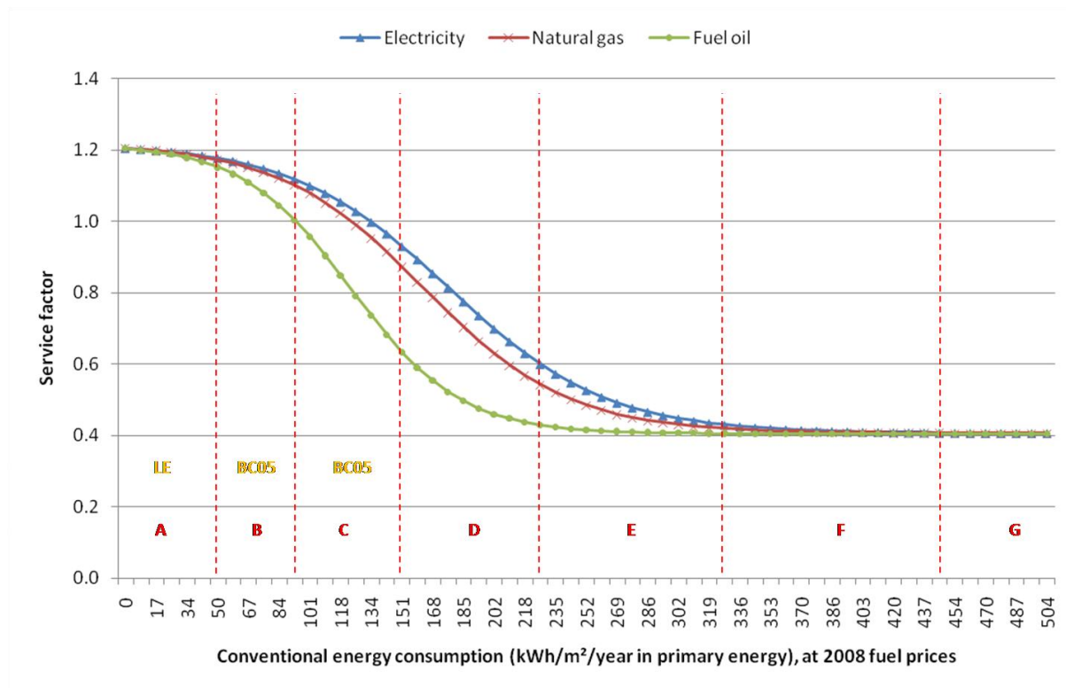
Figure 55: Sufficiency curve (adapted from Allibe, 2009)
