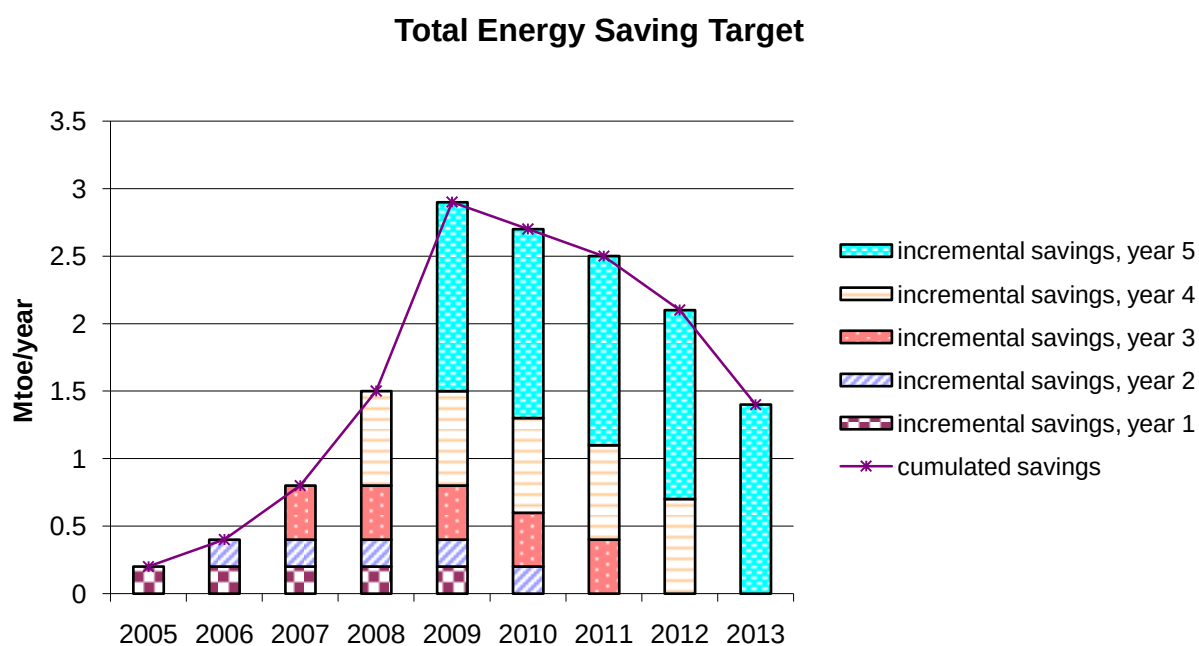
Figure 52: Italian energy saving target
